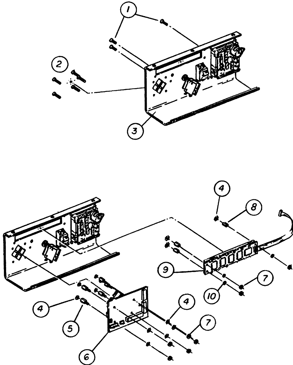
Control Console Assembly - fig. 8
